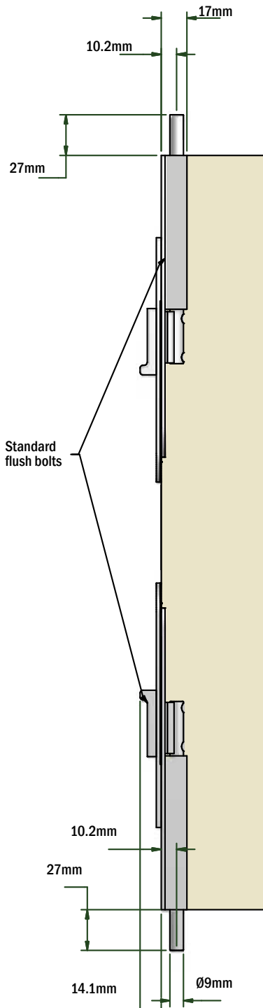
STANDARD FLUSH BOLTS For outward opening doors
