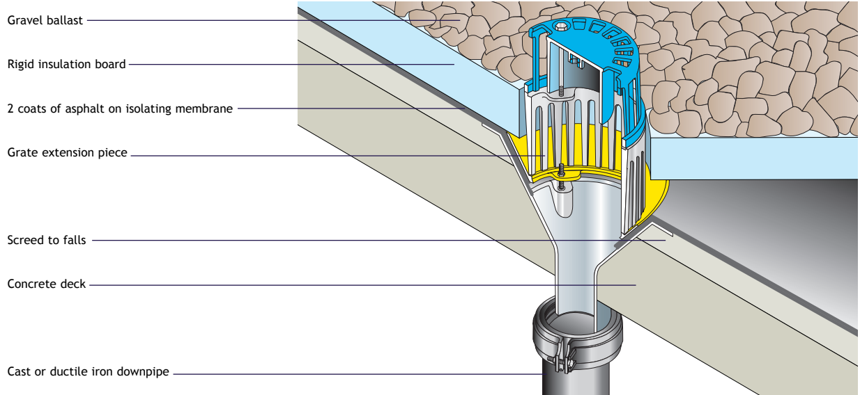
Harmer AV Vertical Spigot Outlet and Extension Piece in Inverted Roof
