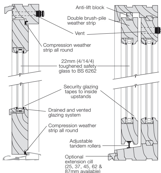
Vertical Section French Style Patio Door, Open Out
