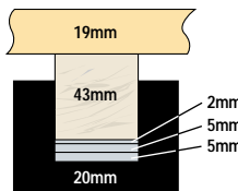
94mm finished floor height
