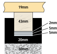
124mm finished floor heights
