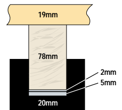
124mm finished floor heights
