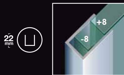
22MM SURFACE PROFILE (allows up to 16mm adjustment)
