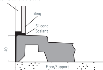
Typical Wall Installation New Continental 40
