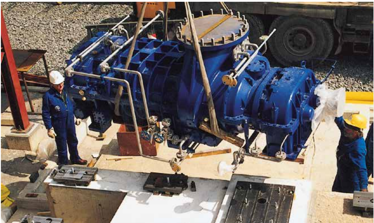
Kaucuk A.S., Kralupy (Czech Republic) Assembly of a process gas compressor VRa 736 L
