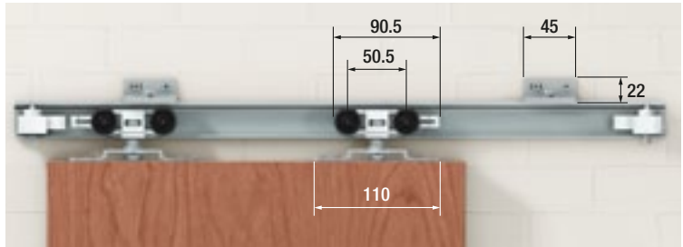
Soffit fixing for two doors. (Mount 2 tracks side by side)
