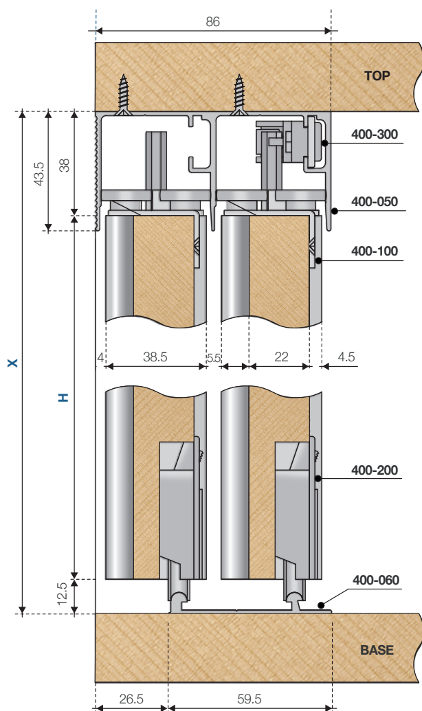
2x Top Guides
