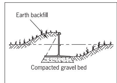
Installation in level terrain, lower elevation
