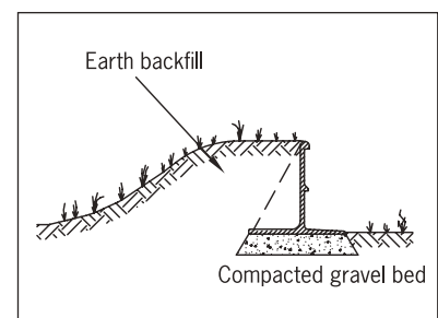
Installation in level terrain, same elevation
