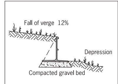
Installation – verge
