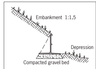
Installation – embankment
