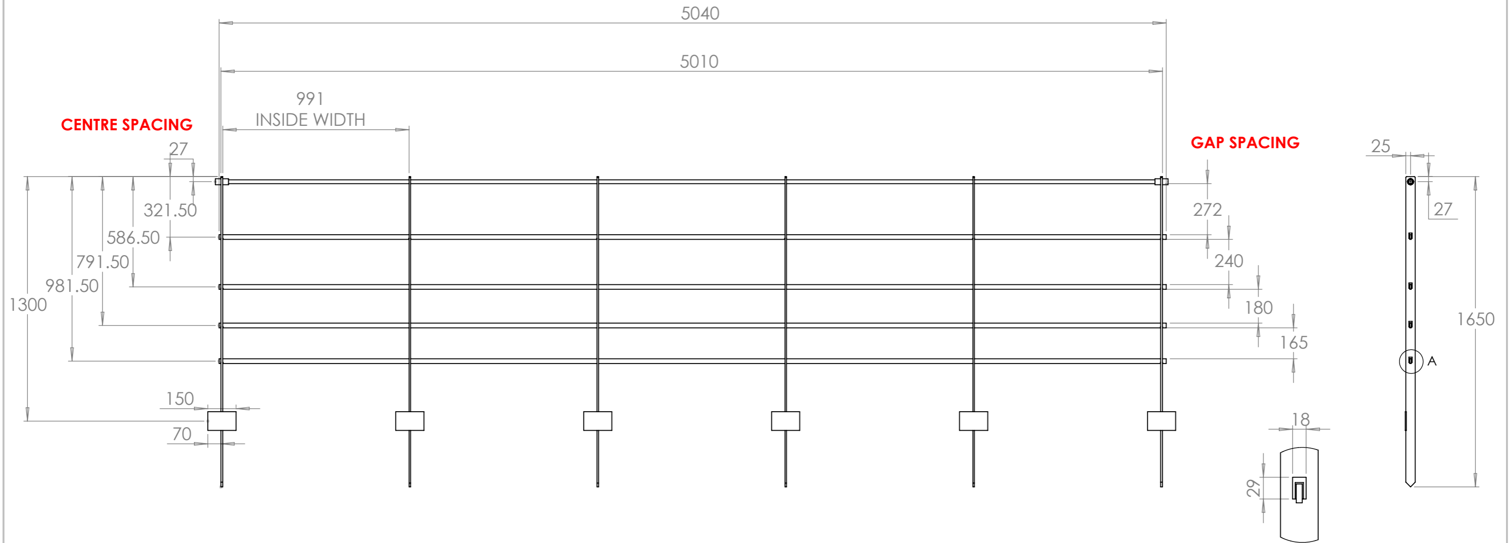
DETAIL A SCALE 1 : 5
