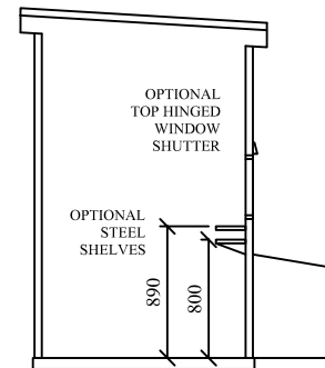
SECTION
