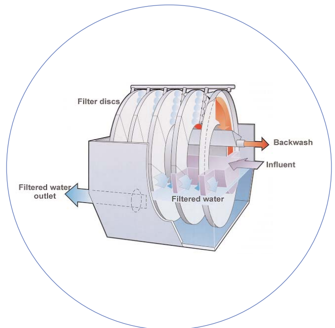
Hydretech® Discfilter Flow Path
