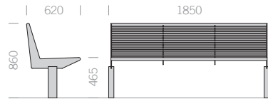
Hocker 1850 Stool bench 1850
