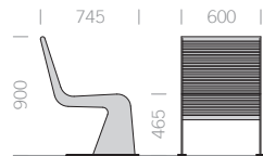
Hocker 1800 Stool bench 1800
