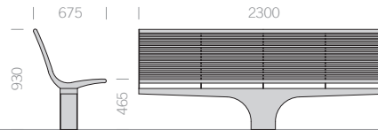
Bank ohne Armlehne Bench without armrests
