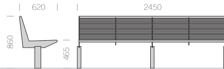
Hocker 2450 Stool bench 2450
