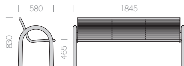
Hocker Stool bench
