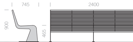
Bank 2400 Bench 2400
