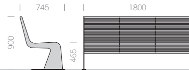
Hocker 2450 Stool bench 2400
