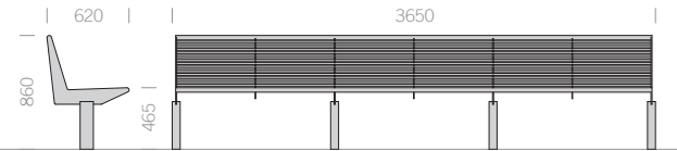
Hocker 3650 Stool bench 3650
