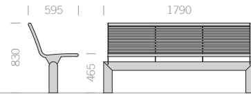
Bank ohne Armlehne Bench without armrests
