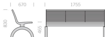
Bank ohne Armlehne Bench without armrests
