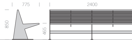
Hocker 2400 Stool bench 2400
