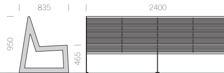
Hocker 2400 Stool bench 2400
