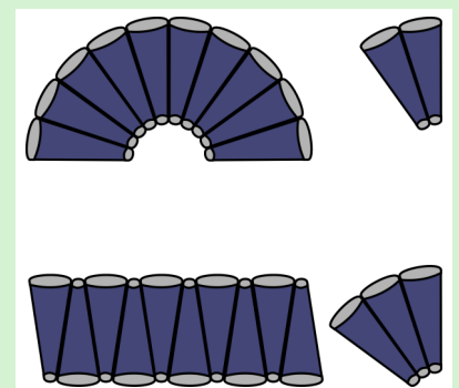
The Velo-Safe design enables flexible layouts to use space well
