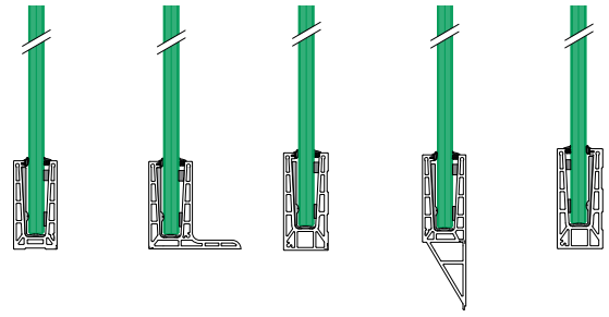
Easy Glass® Pro Top mount / In-floor Easy Glass® Pro F Top mount Easy Glass® Pro Fascia mount Easy Glass® Pro Y Fascia mount Easy Glass® Pro Inverse Fascia mount
