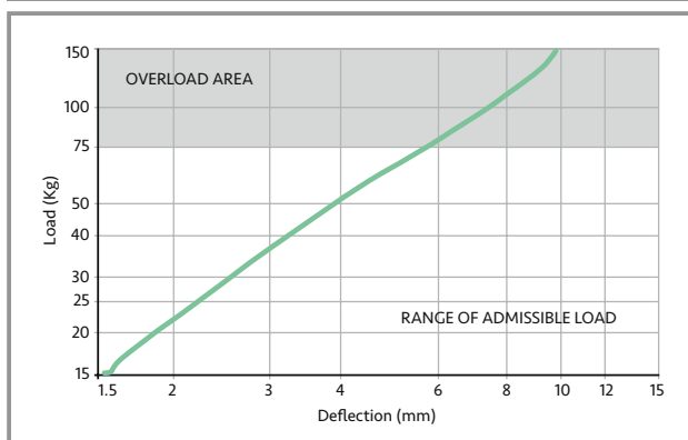
Load Deflection Graph - SH75
