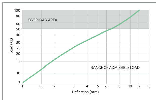
Load Deflection Graph - SH50
