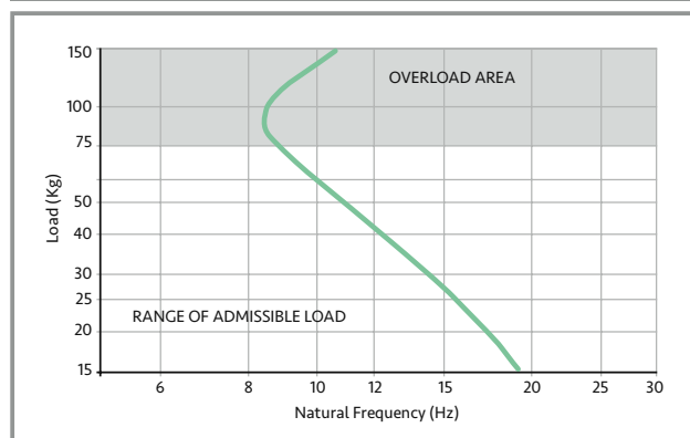
Natural Frequency Graph - SH75
