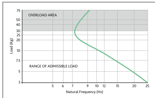
Natural Frequency Graph - SH30
