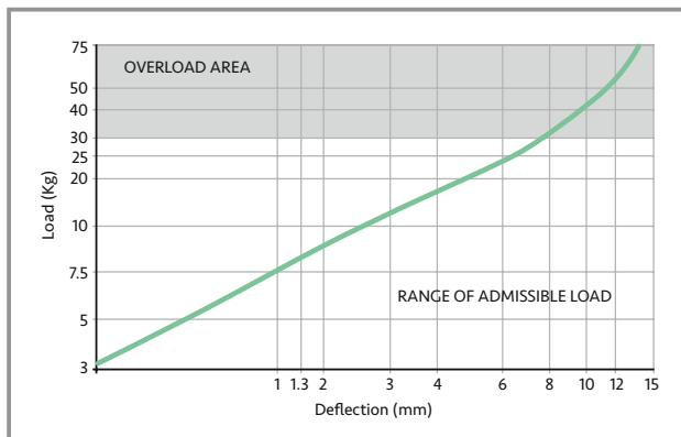
Load Deflection Graph - SH30
