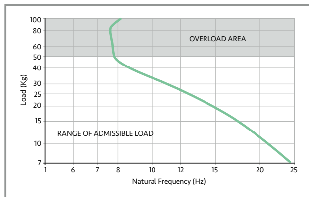
Natural Frequency Graph - SH50
