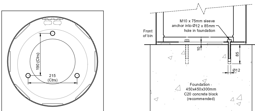
Fixing detail
