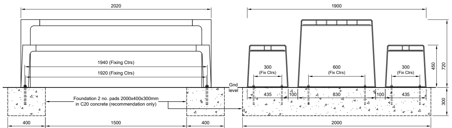
Setting out dimensions
