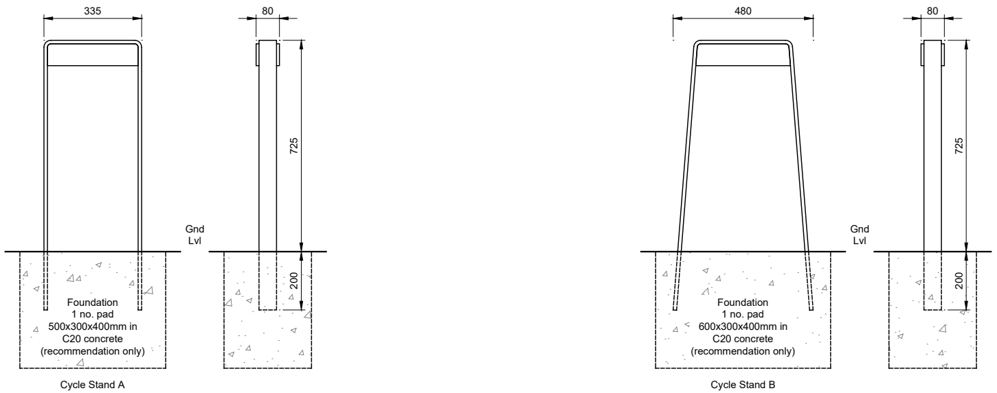
Bike Stands ( Sub-surface Fix Only )
