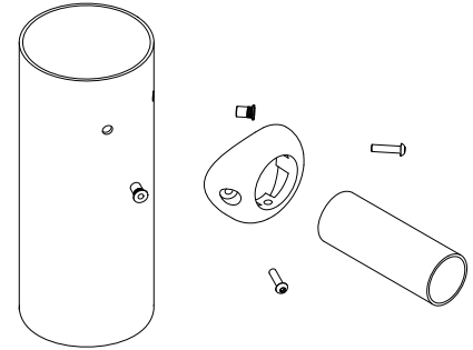
Linx 300 post-to-rail connection
