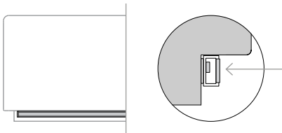
Enlarged cross section showing LED housed in aluminium extrusion with acrylic diffuser
