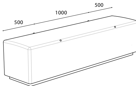
BLYTH 2M 2 balls on each long side
