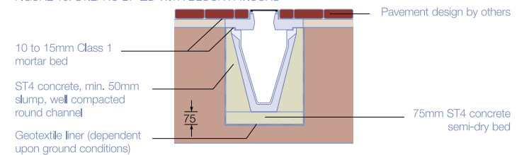
FIGURE 10: STILPRO BP LID WITH BLOCK PAVIOURS
