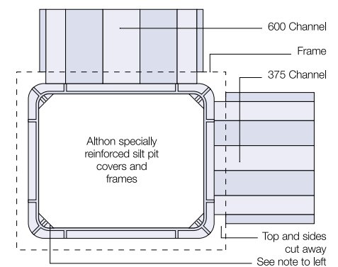
FIGURE 3c: SILT PIT WITH 600 and 525 UNITS
