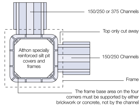
FIGURE 3a: SILT PIT WITH 150 OR 250 UNITS
