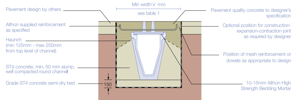
FIGURE 4: FORMA D400 UNIT
