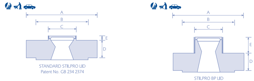
Figure 2: Standard Althon Lid Types scale 1:10
