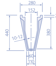
CH 150 overall effective length 2000mm
