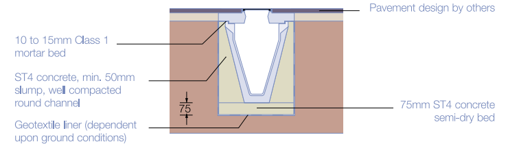
FIGURE 10: STILPRO BP LID WITH BLOCK PAVIOURS
