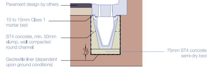
FIGURE 9: STANDARD STILPRO LID WITH ASPHALT
