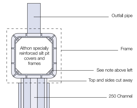
FIGURE 3e: SILT PIT WITH CHANNEL AND OUTFALL PIPE
