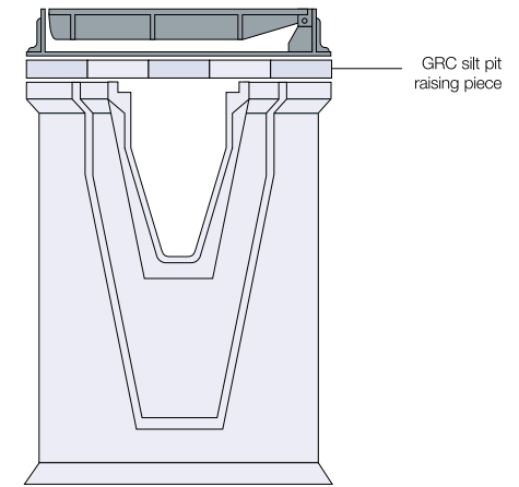
FIGURE 3d: SILT PIT WITH GRC RAISING PIECE
