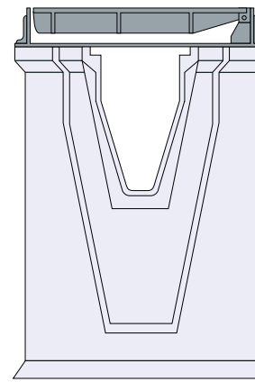
FIGURE 3: SILT PIT
