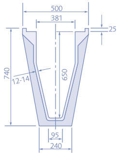
CH 375 overall effective length 1500mm
