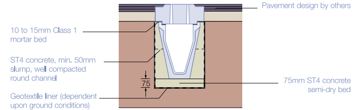
FIGURE 8: KHB LID WITH ASPHALT
