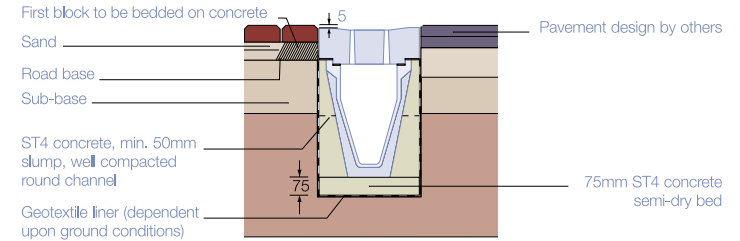
FIGURE 7: JS3 LID WITH ASPHALT
