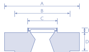
STANDARD STILPRO LID Patent No. GB 234 2374
