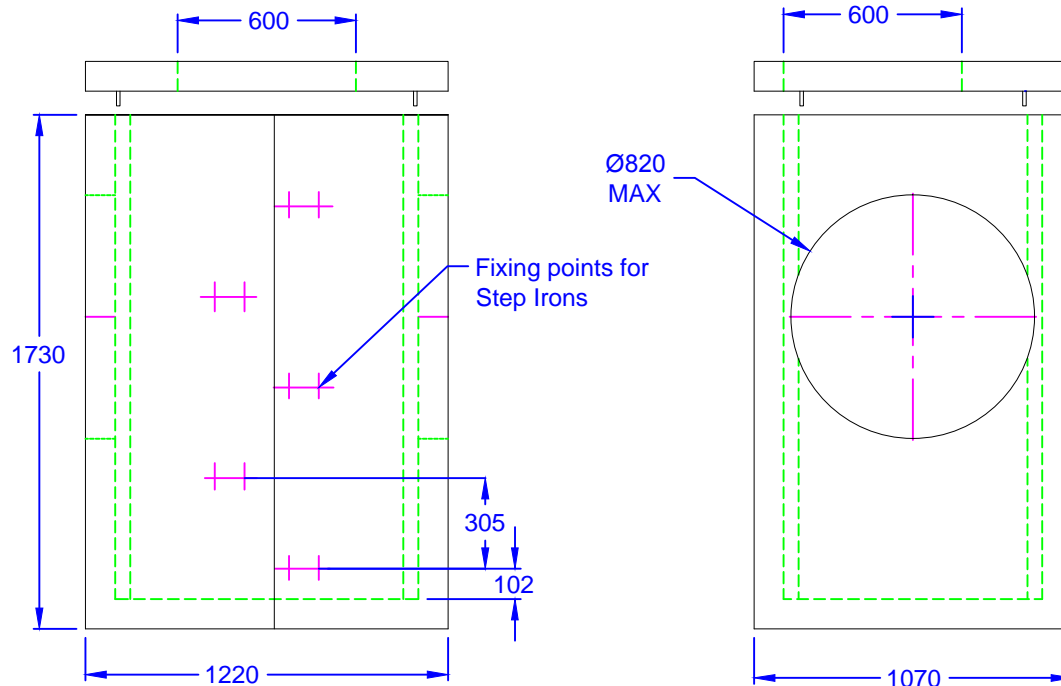
SIDE VIEW OF CHAMBER
