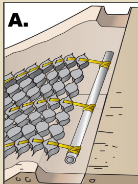
"Deadman" Pipe
