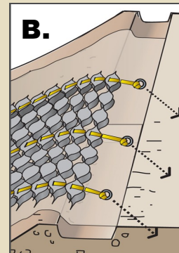
Earth anchors
