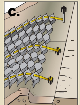
ATRA Anchors
