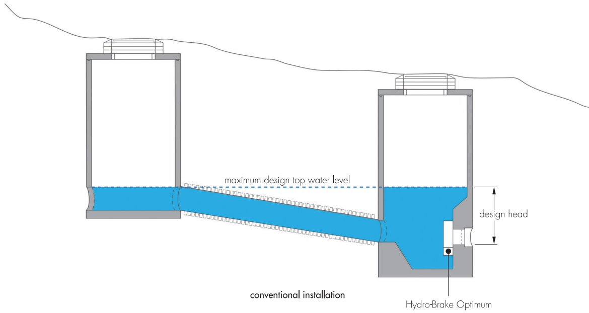
Figure 3 Typical applications and design head
