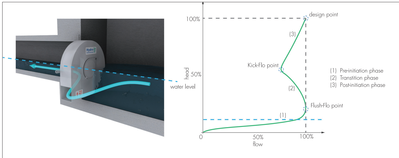
Figure 4 Pre-initiation phase
