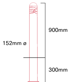
▲ Shown 152mm ø, 900mm high, Root Fixing, available only in size shown.
