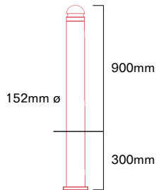
▲ Shown 152mm ø, 900mm high, Root Fixing.
