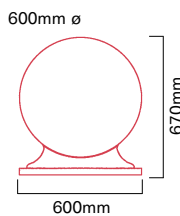
▲ ASF 127 Base Plate Fixing
