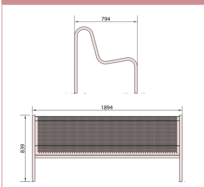
STATION SEAT
