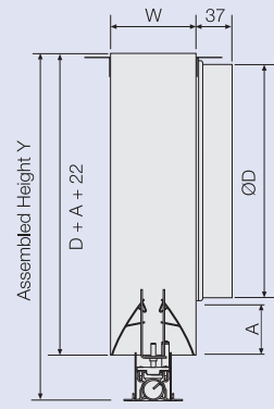
Assembled Height Y = VSD35 (D + A + 71) Extension A = 125, 150, 200
