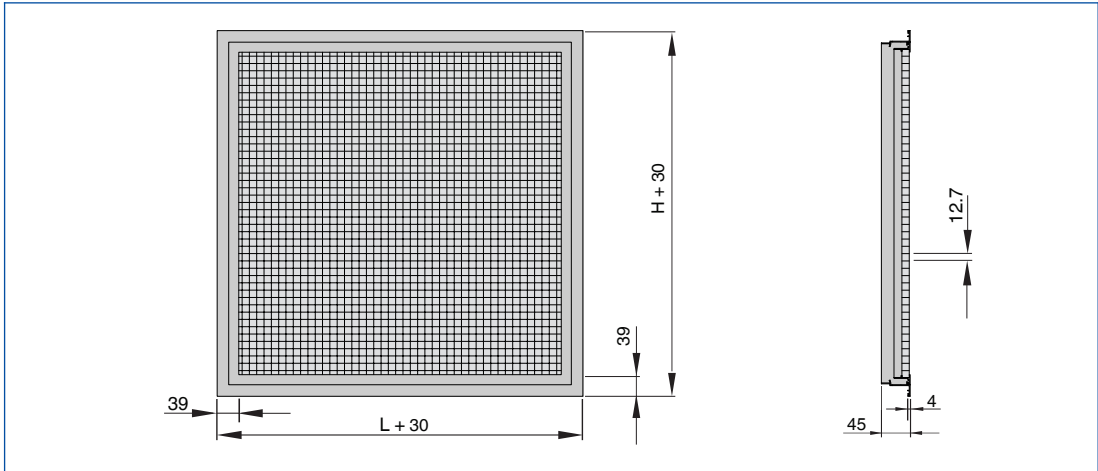
RC-AE, 39 mm wide front border
