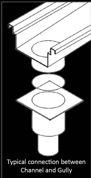
Typical 3071EF / 3010 Channel to Vertical Outlet Gully
