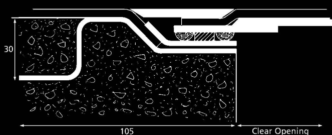
Type 4300 Vinoseal Cover
