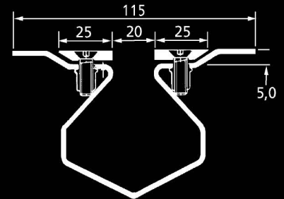
Type 3610V with built in fall Type 3611V 50mm constant depth
