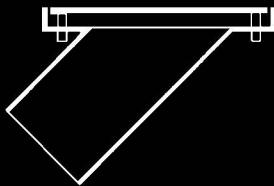
Type 5600 Rodding Eye 45° x 110 Spigot
