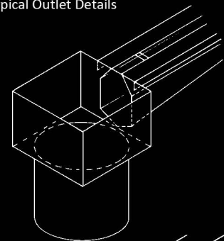
Typical Outlet Details
