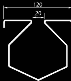
Type 3620 with built in fall (Jumbo Compact)
