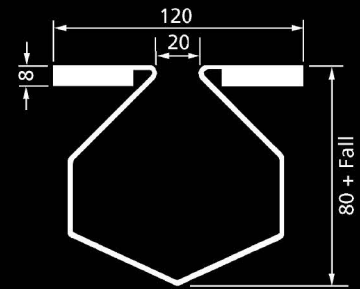
Type 3630 with built in fall (Reinforced Jumbo Compact)
