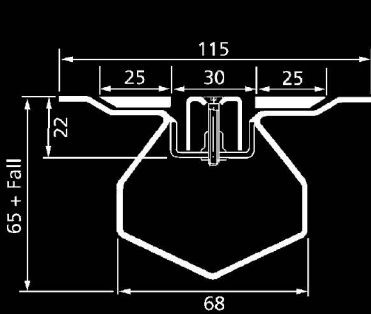
Type 3610VG with built in fall Type 3611VG 50mm constant depth
