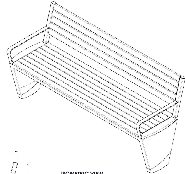
ISOMETRIC VIEW SCALE 1:10
