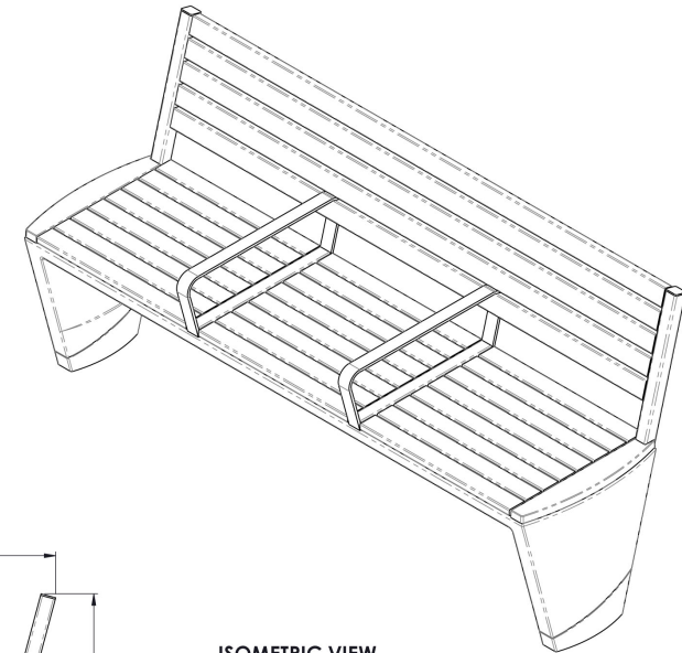
ISOMETRIC VIEW SCALE 1:10
