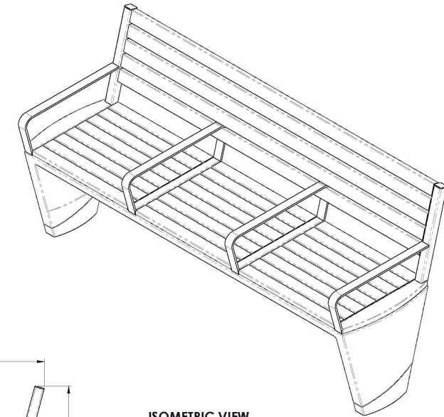
ISOMETRIC VIEW SCALE 1:10
