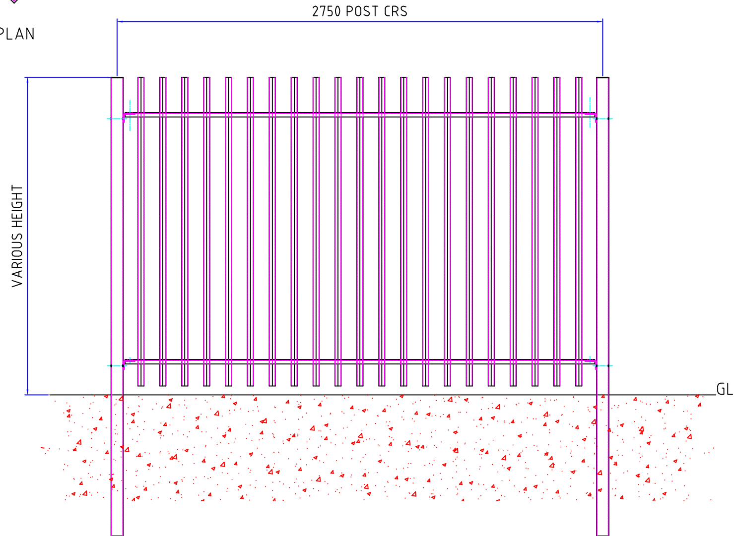
TYPICAL PANEL ELEVATION
