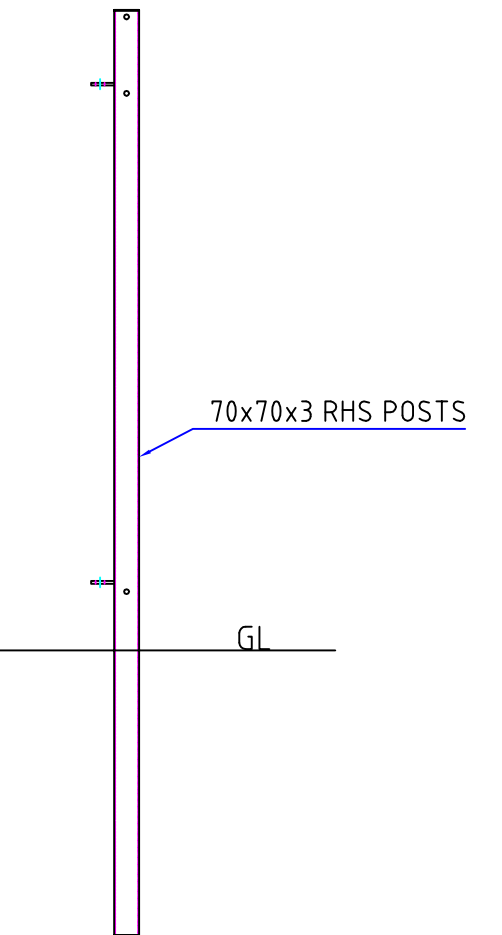
TYPICAL LOOSE CLEAT POST ELEVATION
