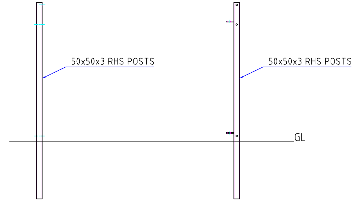
TYPICAL LOOSE CLEAT POST ELEVATION
