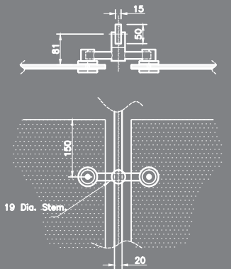
Special Barrel Glass Fitting (L7)
