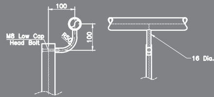
Offset Radius Bracket (BB3)
