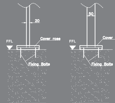
Standard Top Fixing (TF5)
