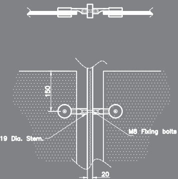
Inline Banjo Glass Fitting (L4)
