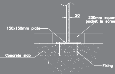
Top Fixing - Screed Fix (TF6)
