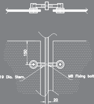
Standard Barrel Glass Fitting (L5)
