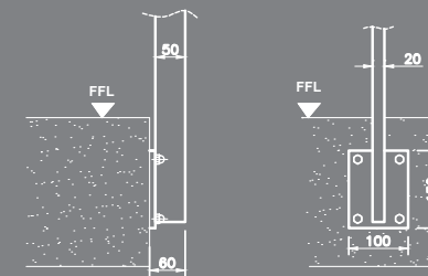
Standard Side Fixing (Welded) (SF4)
