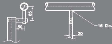
Standard Offset Barrel Bracket (BB4)
