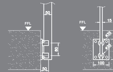
Special Side Fixing (SF7)
