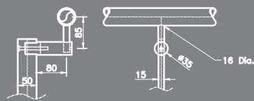
Special Offset Barrel Bracket (BB7)
