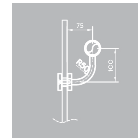
Offset Radius Bracket (BB3)
