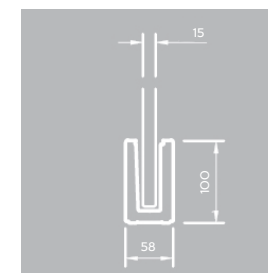
Aluminium Channel (BC1)*
