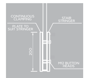
Clamp Plate to Steel Stringer (SF8)*
