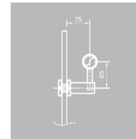
Offset barrel Bracket (BB5)
