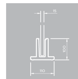
Aluminium Channel (BC4)*
