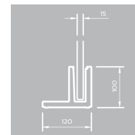
Aluminium Channel (BC2)*
