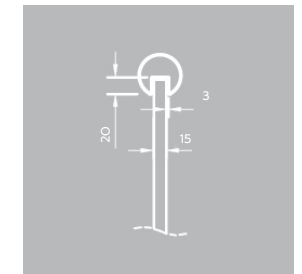
Slotted Handrail (BB6)
