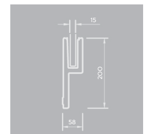
Aluminium Channel (BC3)*
