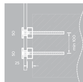
Slimline 2-Point Side Fixing (SF6)*
