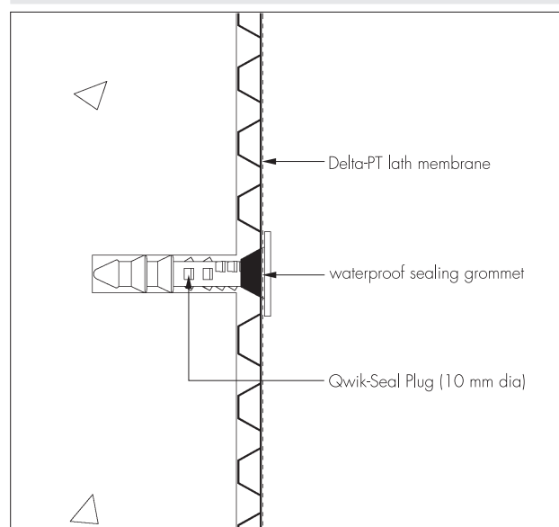
Figure 4 Delta Qwik-Seal Plug fixing detail
