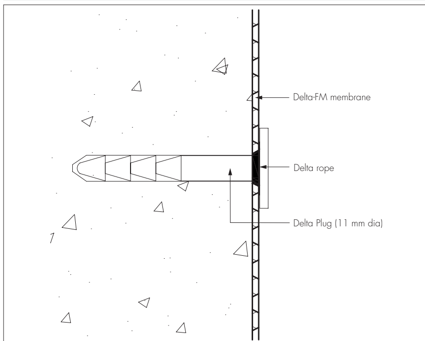
Figure 3 Delta Plug fixing detail
