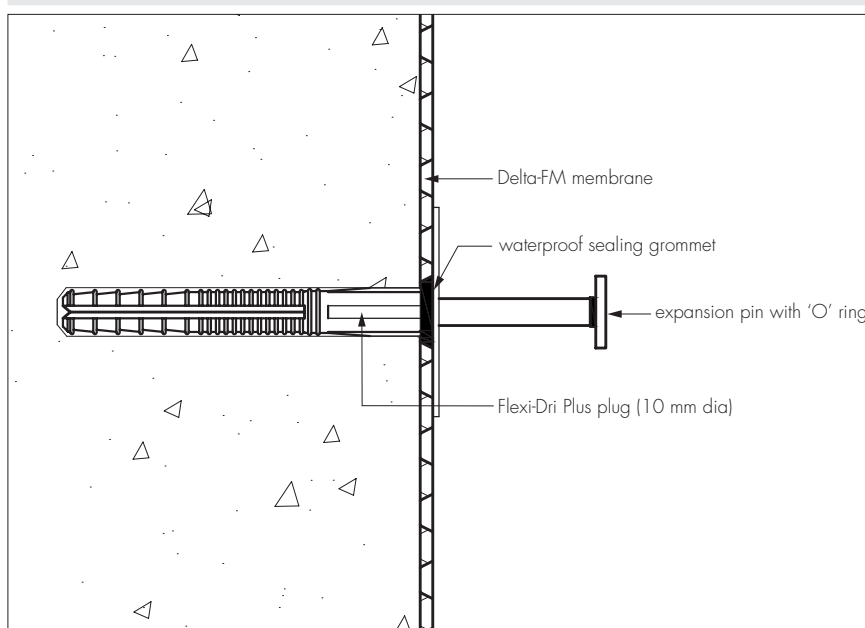
Figure 1 Flexidri-Plus — Fixing Plug detail
