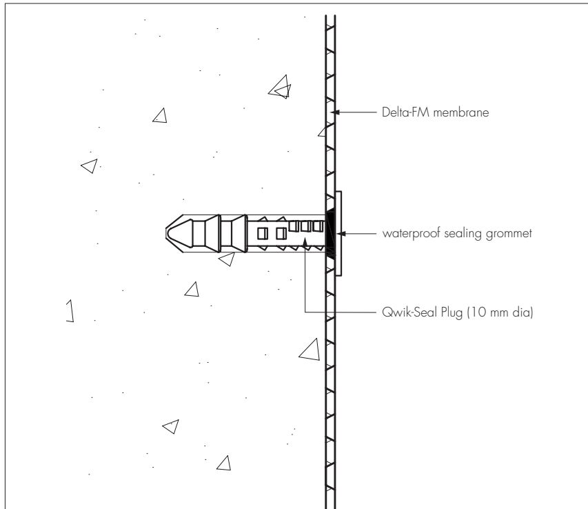
Figure 3 Delta Plug fixing detail
