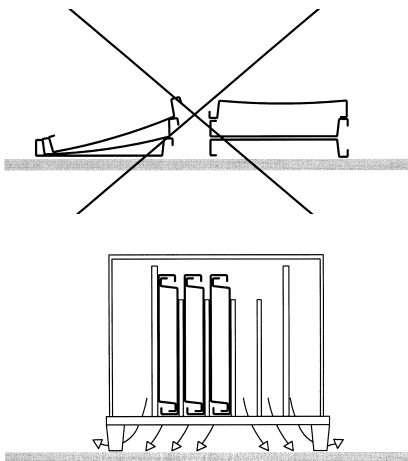
Transportation and storage of panels
