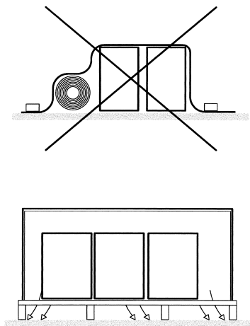
Transportation and storage of coils
