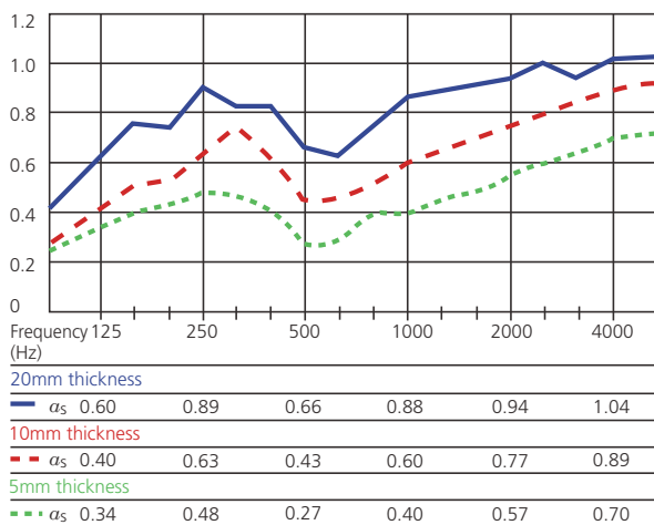
Sound absorption coefficient \alpha_s
