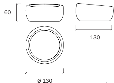
russes J 130 | 700 kg | 210 L
