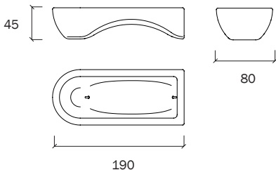
waves J (planter) | 640 kg | 295 L
