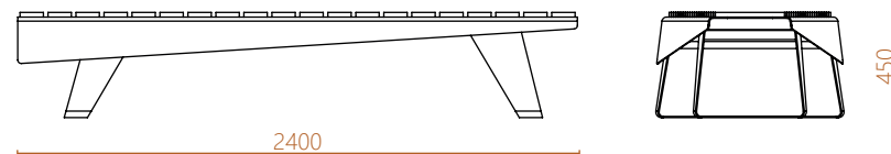
Bench - North South arlo-04-a
