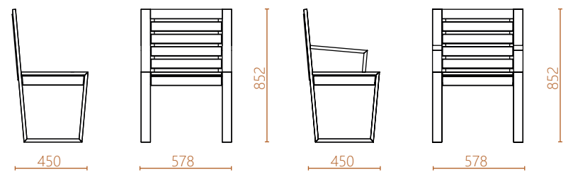
Chair with arms (right) arlo-01-f
