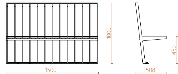
Bench - High Back arlo-09-a
