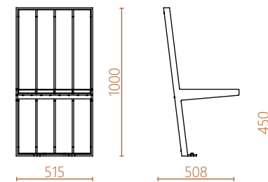
Stool - High Back arlo-09-c
