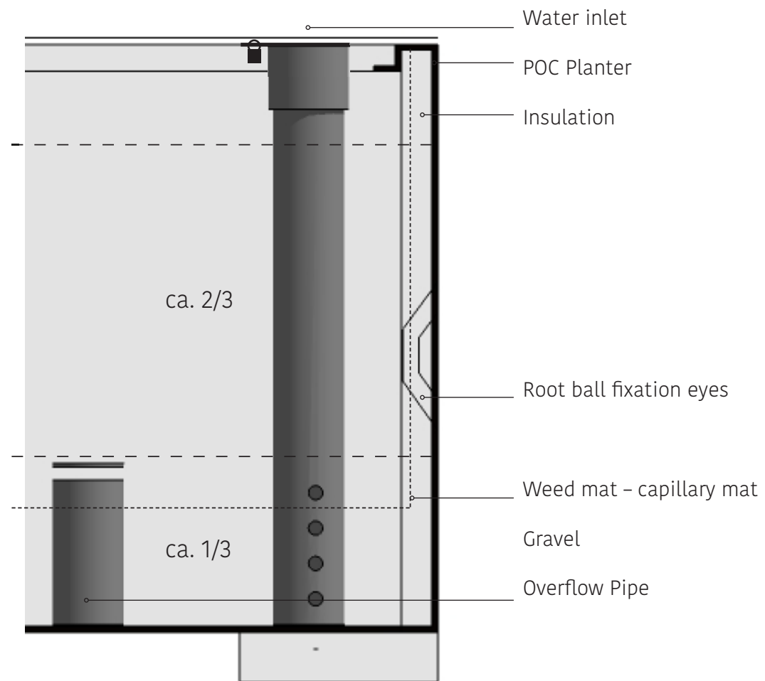
Cross section
