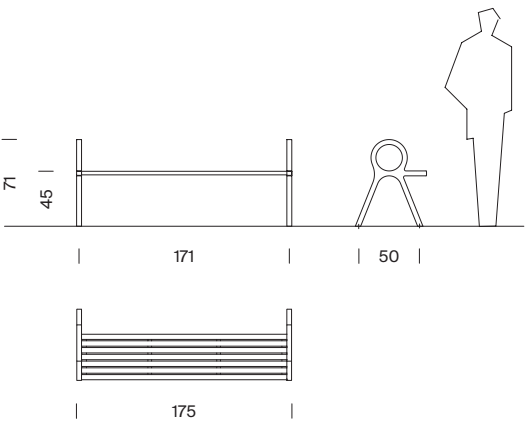
Perisphere bench one unit without backrest
