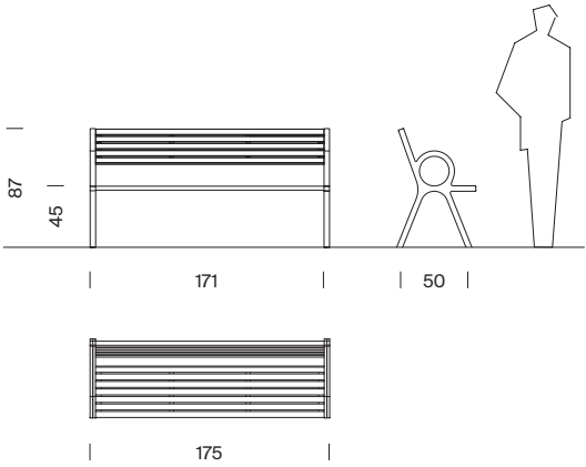
Perisphere bench one unit with backrest
