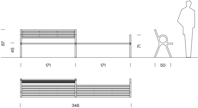
Perisphere bench two units with initial backrest
