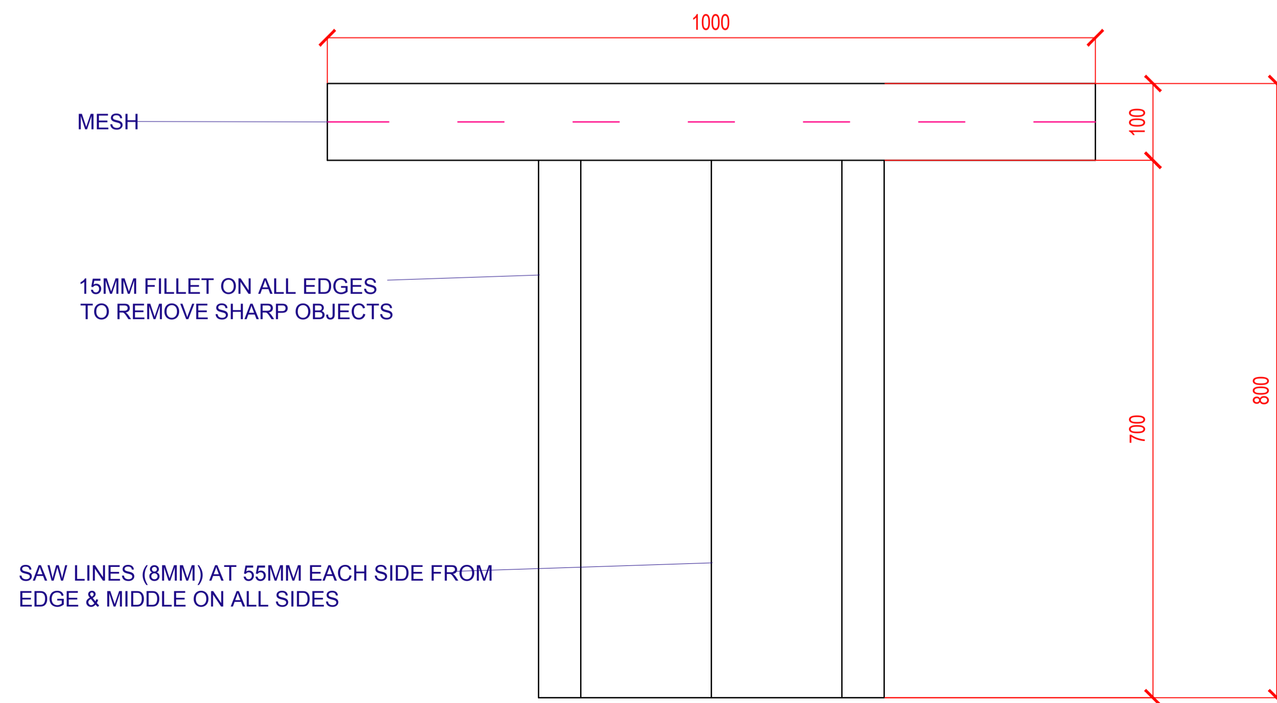
Front View Scale 1:5
