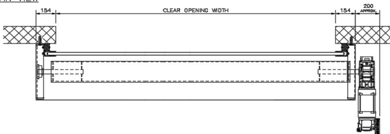
ENLARGED JAMB DETAIL
