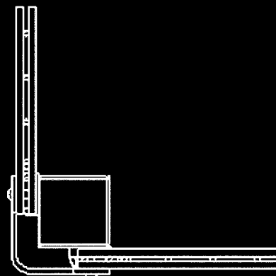
Standard Goal Recess Safety Cover Strip
