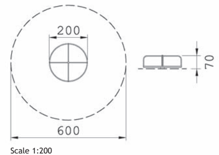
Scale 1:200
