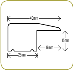
Rebated L Section 15mm Rebate
