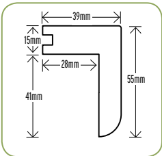
Nosing (grooved) 15mm
